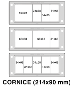
CORNICE (214x90 mm)
