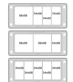
CORNICE (214x90 mm)
