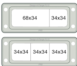
CORNICE (134x52 mm)
