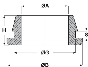
DKA 12/16/19,5-2
